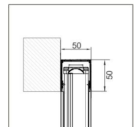
BORA UP MIDI 35/35
