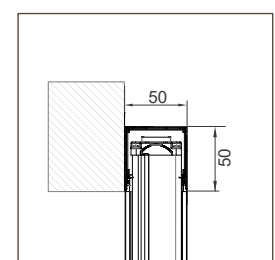
BORA UP MIDI 50/50
