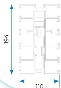
6 GUIA CENTRAL 5° CARRIL PANEL MÓVIL
